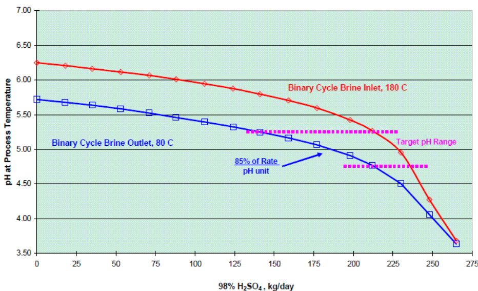
Characteristic pH Modification Curve for Pumped-well Binary-Cycle
